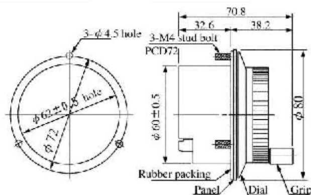
Panel Cutout
