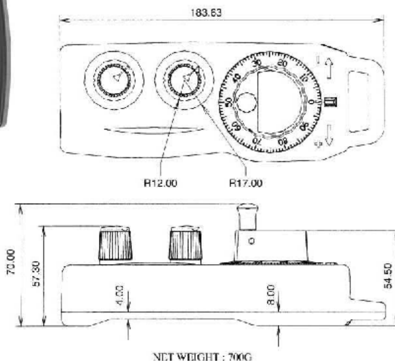
EHDW-B~C EXTERNAL DIMENSIONS
